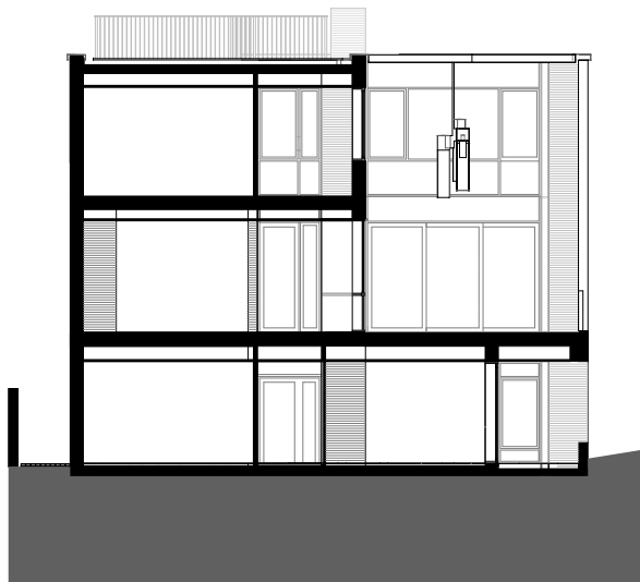
SECTION EAST WEST 1:200
